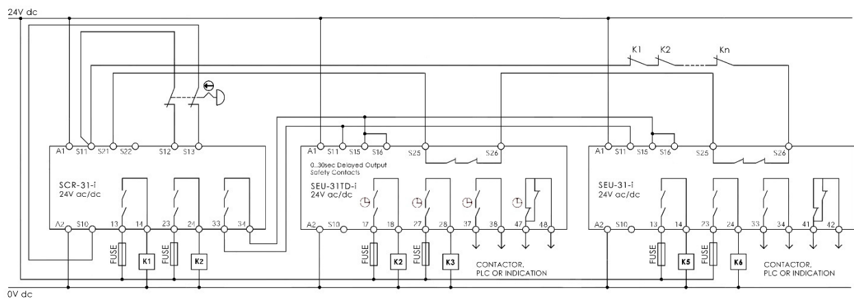
Fig.1 SCR-31-i, Dual Channel, E-Stop, Manual Reset with Expansion Unit SEU-31TD-i
