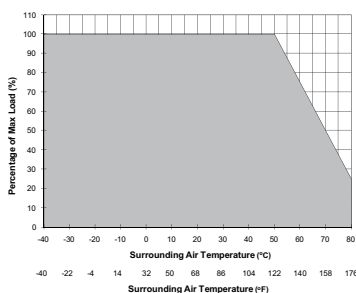
Power Derating Curve for Redundancy Module
