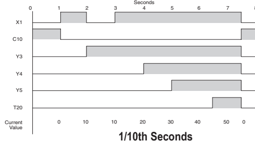
Timing Diagram
