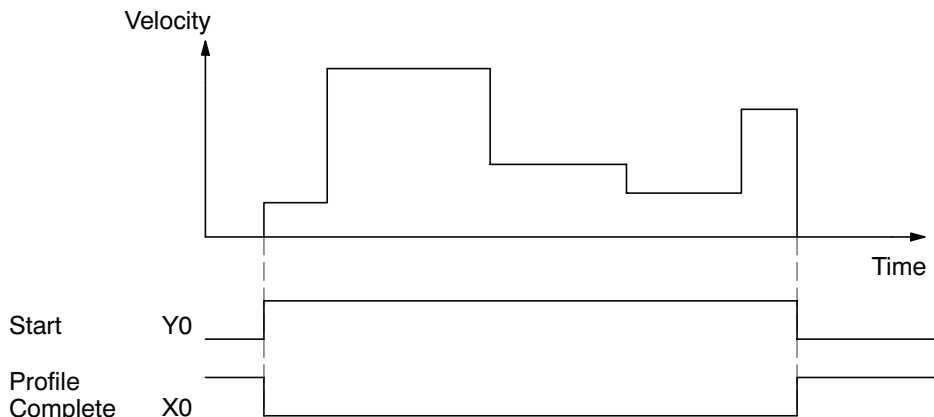
Velocity Profile
