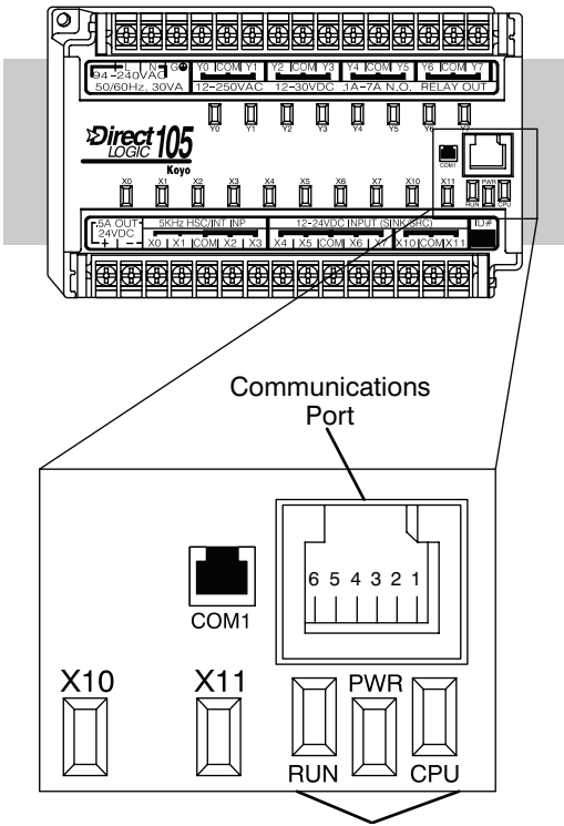
CPU Status Indicators
