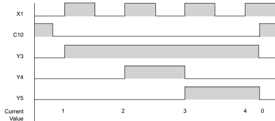
Counting diagram
