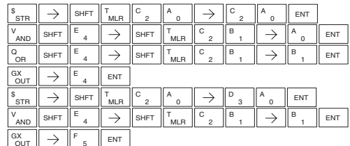
Handheld Programmer Keystrokes (cont'd)
