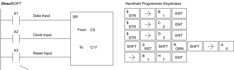
Inputs on Successive Scans
