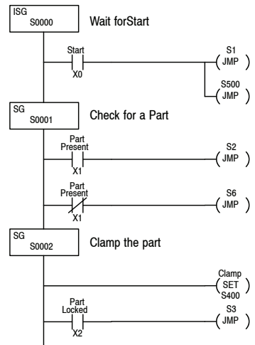
Ladder Representation
