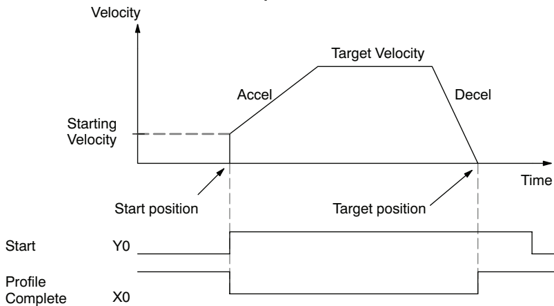
Trapezoidal Profile
