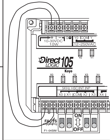
F1-130DR, F1-130DD-D (DC-powered versions)
